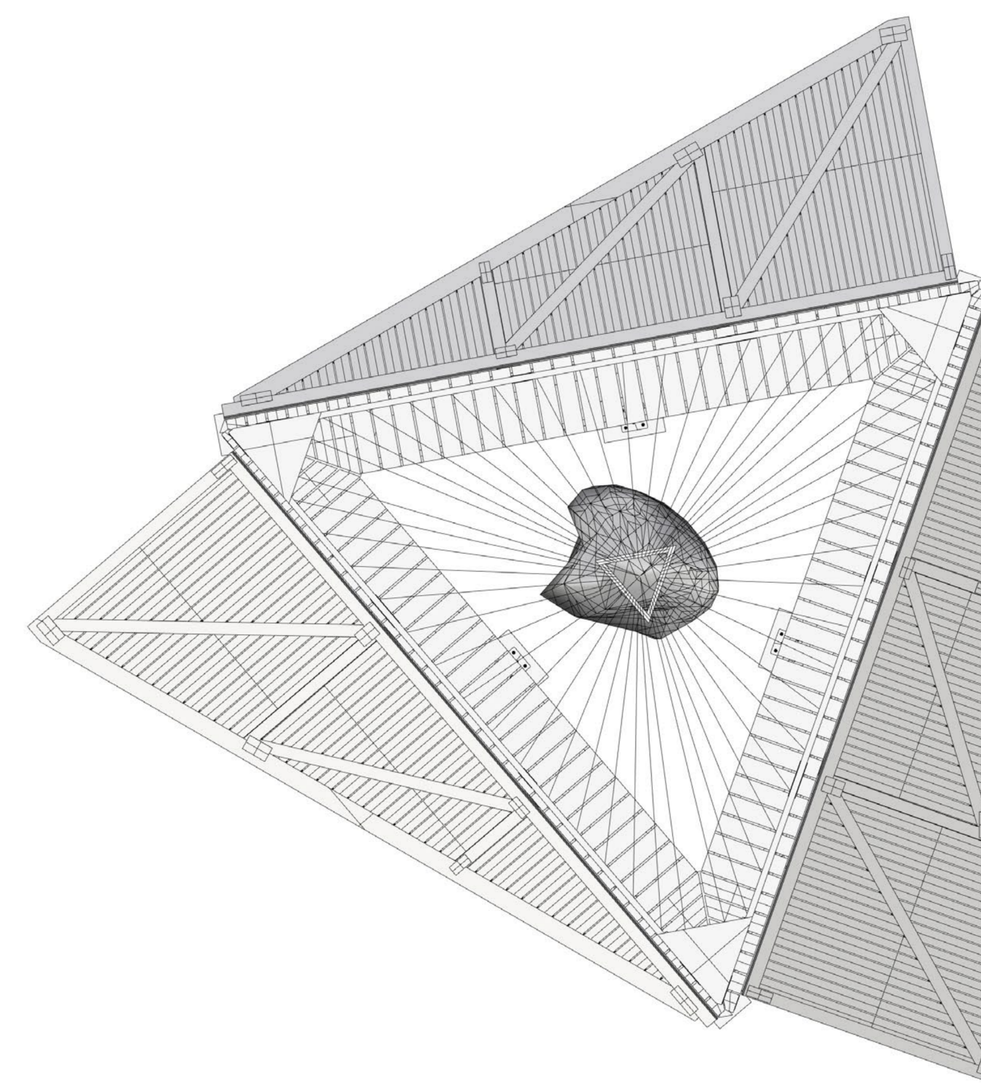
Plan
